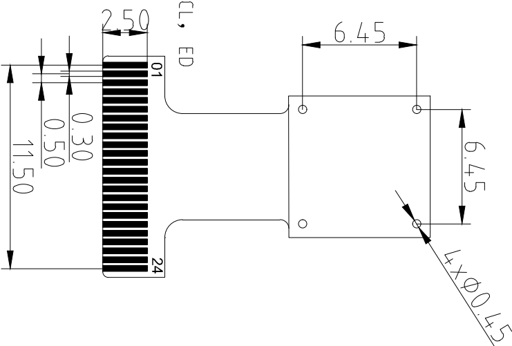
BOTTOM VIEW
